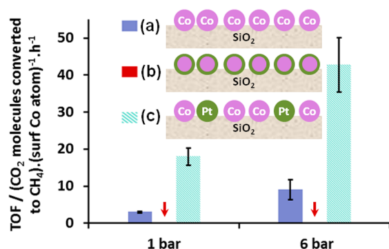
Figure 2. Turnover frequencies at 1 and 6 bar total pressure for the production of CH_4 during catalytic CO_2 hydrogenation ( 1:3 CO_2:H_2 ) at 200^\circ C for three catalyst samples: (a) 10 nm Co NPs supported on MCF-17 mesoporous silica, (b) 11 nm Co–Pt binary NPs supported on MCF-17, and (c) 10 nm Co and 12 nm Pt NPs mixed in solution and subsequently supported on MCF-17. The red arrows denote the position of the data points for the Co–Pt binary NP sample (indicating only trace amounts of CH_4 ). Schematic inset indicates overall structure of each sample.
